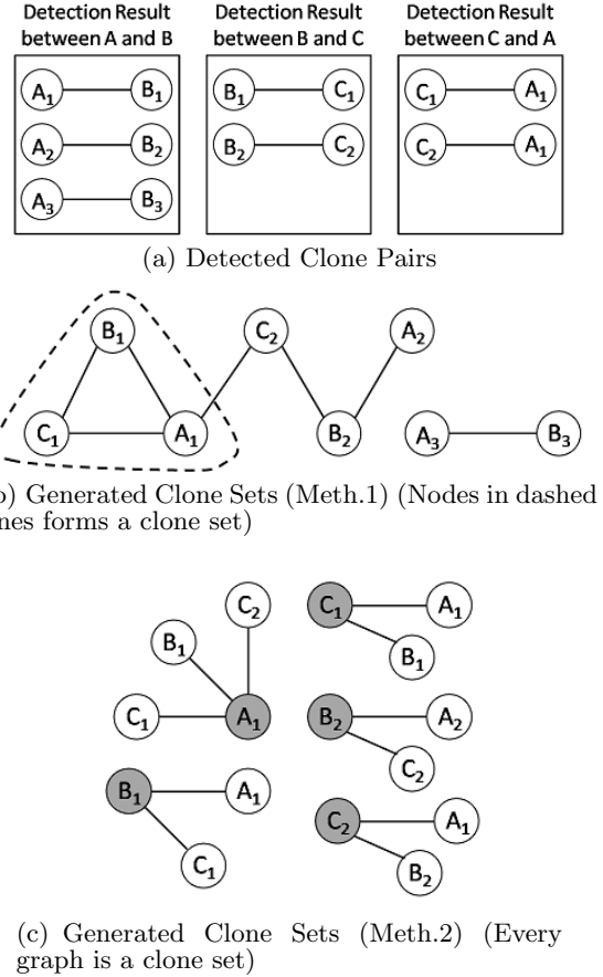
Figure 2: Simple Example of Clone Set Generation (In this example, we extract clone sets that include three or more code fragments)
