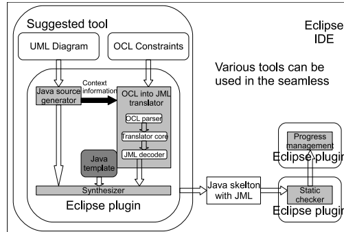
図 1 Tool implementation as Eclipse plugin
