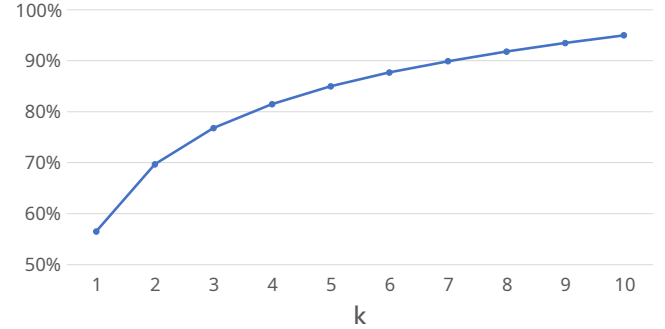
Pass@ k
