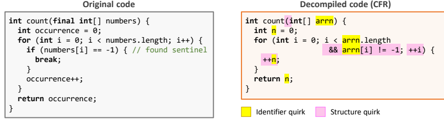
Fig. 1: Example of decompilation quirks in Java
