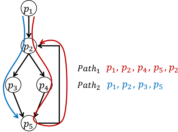
Figure 3.4: Example of path selection for test-case generation
