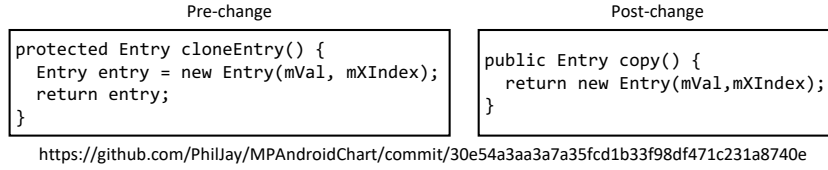
Fig. 3: An example of API change detected by APIDiff alone
