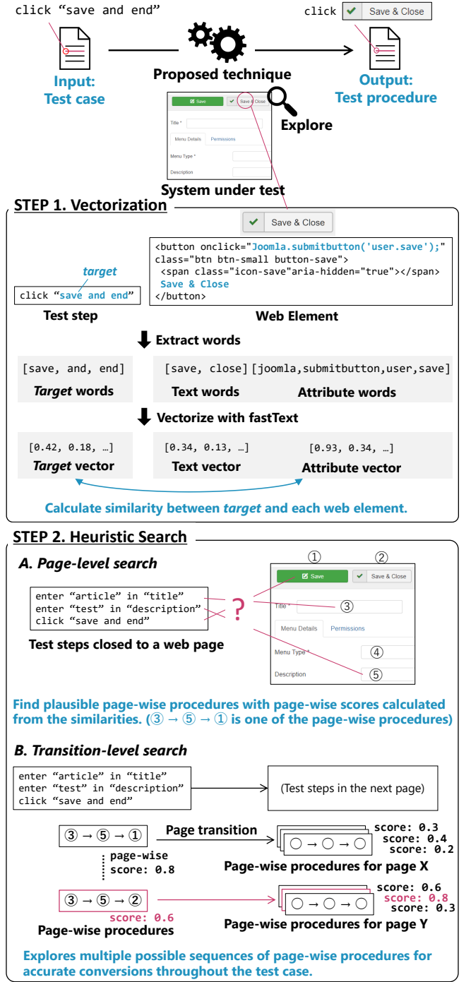
Fig. 2. An overview of our approach
