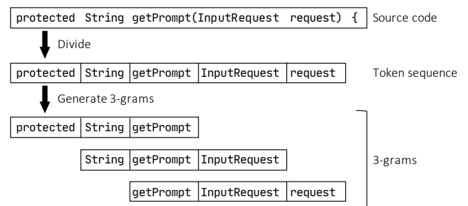
Fig. 3: Example of generating 3-grams
