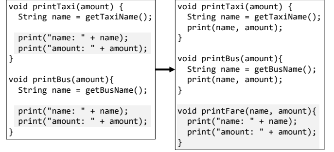
Fig. 1: Extract method refactoring
