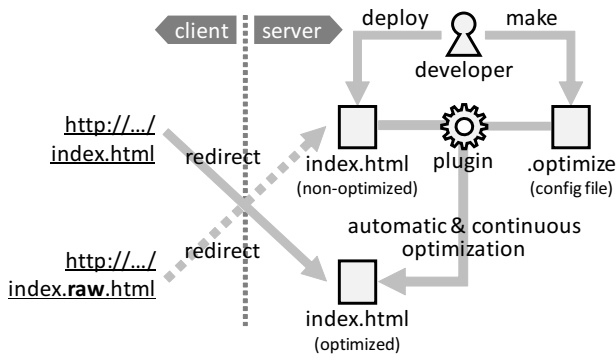
Fig. 1. Processing flow of size optimization plugin
