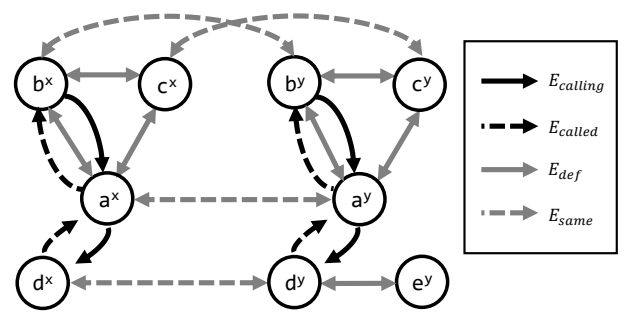
Figure 5: The graph constructed from source code
