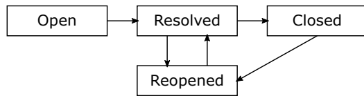
Fig. 1. A Simplified Life Cycle of a Defect Report on JIRA
