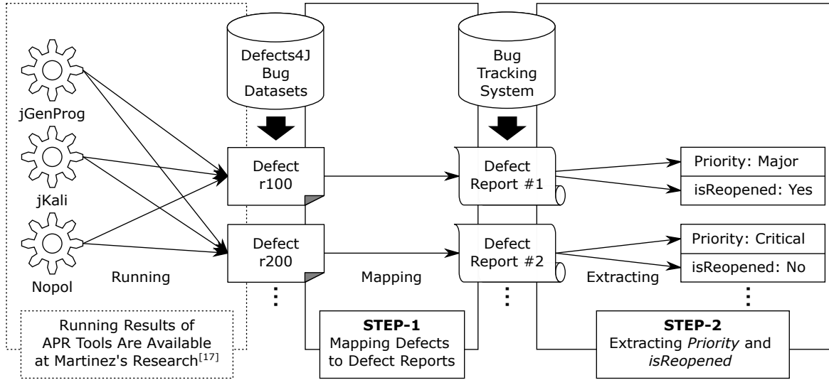
Fig. 2. The Overview of Investigation Method
