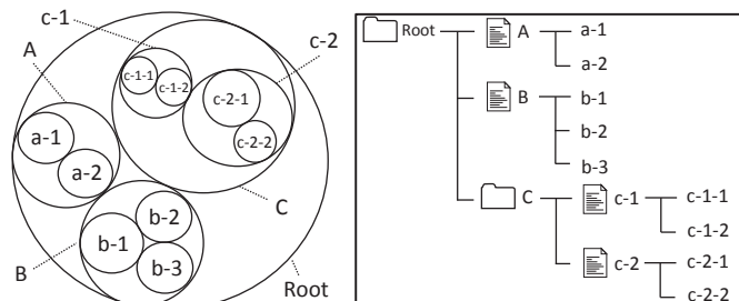
Fig. 1. Example of Circle Packing
