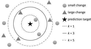
Fig. 3. The k-NN Algorithm
