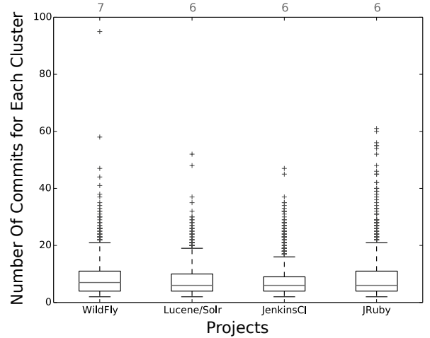
Fig. 4. The Distribution of the Number of Commits for Each Cluster
