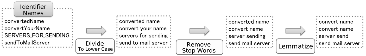
Fig. 3. An example of modifications to the source code
