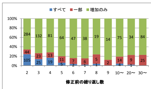
(c) ArgoUML
