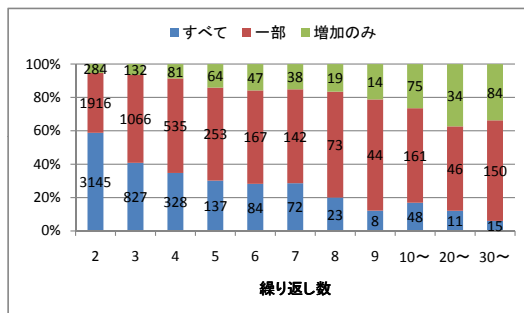
(c) ArgoUML
