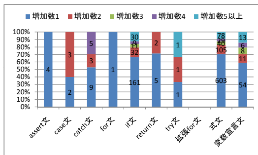
(c) ArgoUML
