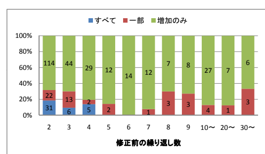
(b) Ant
