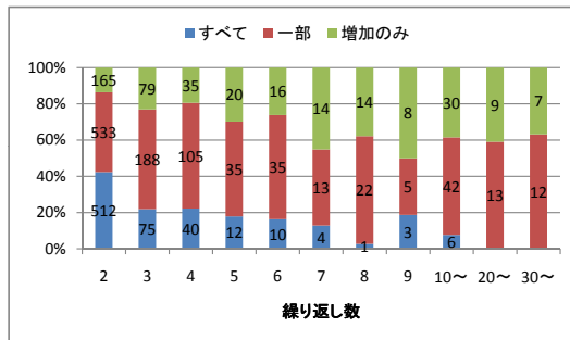
(a) jEdit
