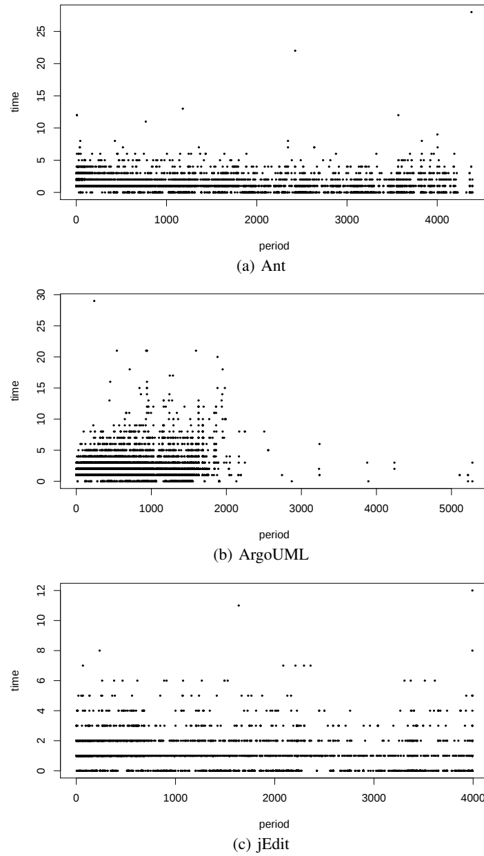
Fig. 7. Relationships between survival period and the number of modifications. Y-axis is the number of modifications, and X-axis is survival period.
