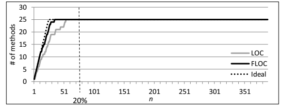
(b) Lines Of Code
