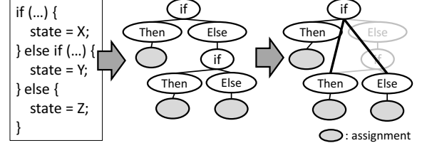
Figure 3. Transformation of else-if Statements
