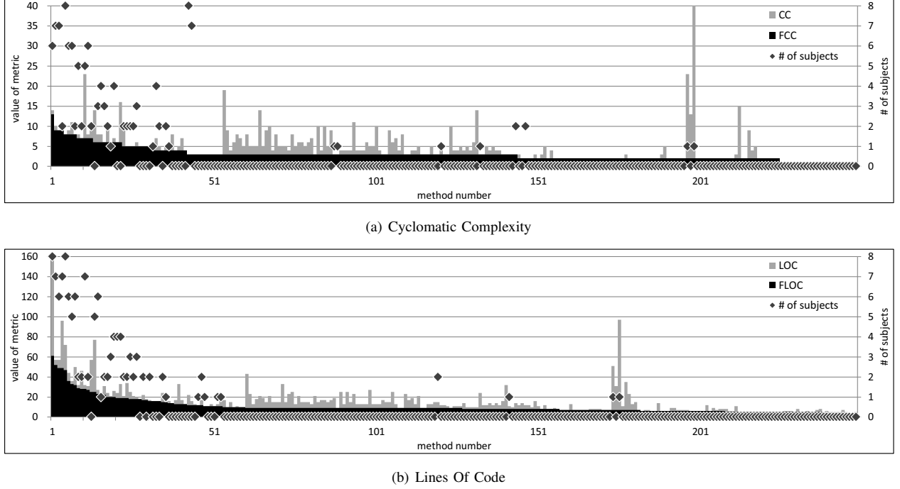
Figure 10. Relationship between Metrics Value and The Number of Subjects
