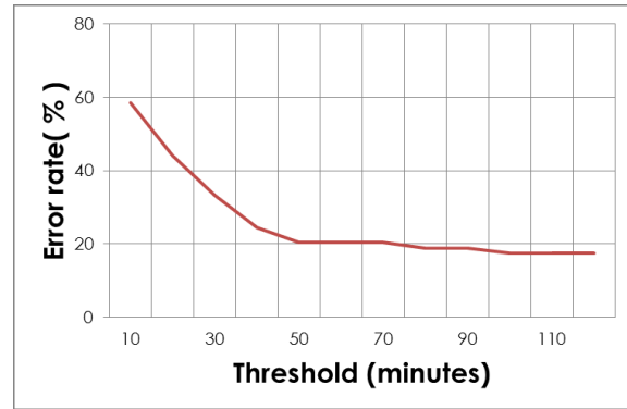
Figure 6. Magnitude of the error rate in application development
