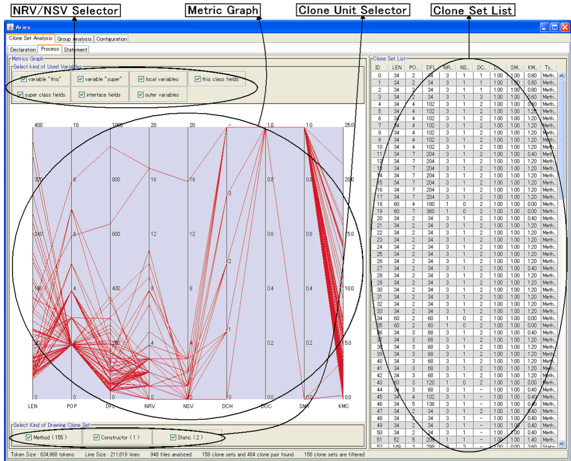
図 2: Main Window
