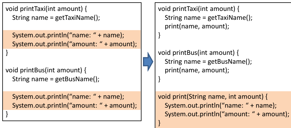
Figure 9: An Example of Extract Method
