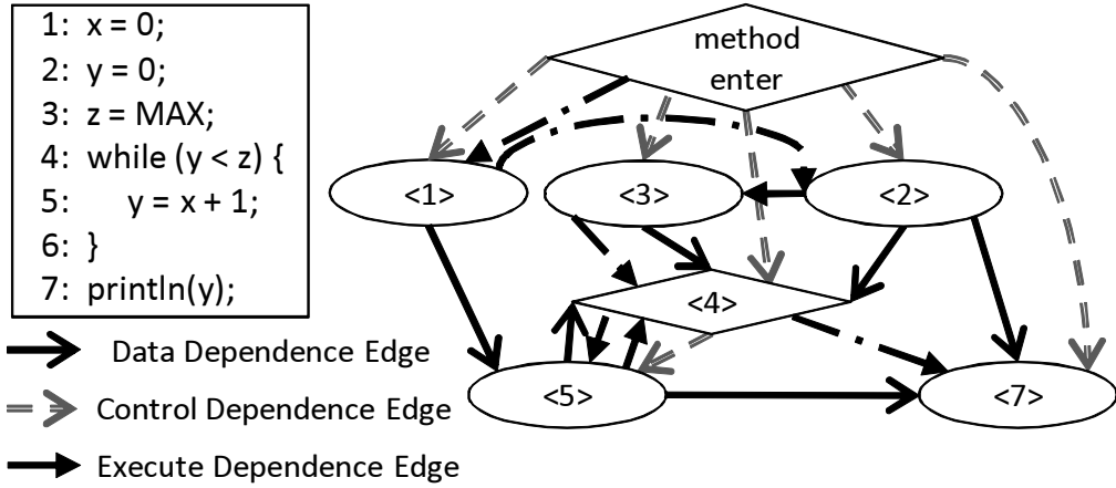
Figure 2: An Example of PDG with Execute Dependence Edges
