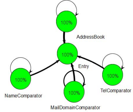
Figure 7. Result of unit testing in Personal Telephone Directory
