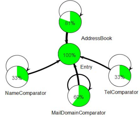
Figure 8. Result of static checking in Personal Telephone Directory
