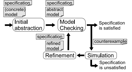
Figure 1 General CEGAR Algorithm
