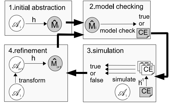
Figure 2 Our Proposed Algorithm
