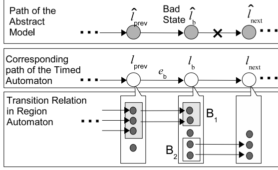
Figure 6 Counter Example
