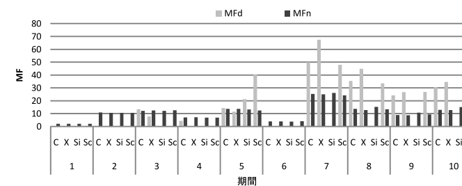
(c) NatMonitor
