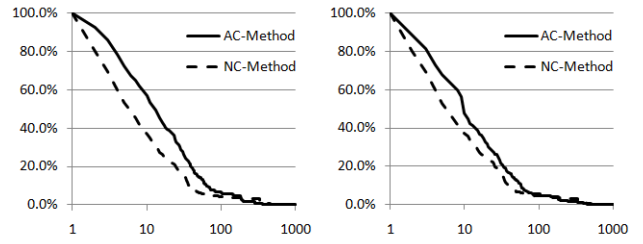
(a) ccf
