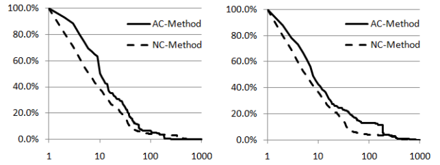
(c) sim
