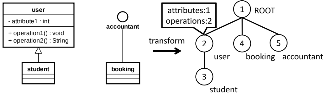
Figure 8: Tree Construction
