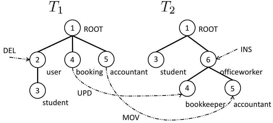
Figure 6: Annotated Trees
