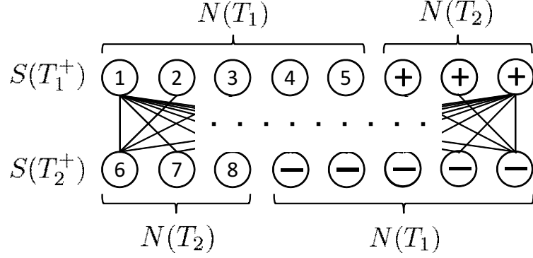
Figure 9: Bipartite Graph
