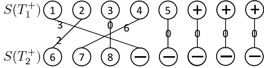
Figure 10: Pruning Problem
