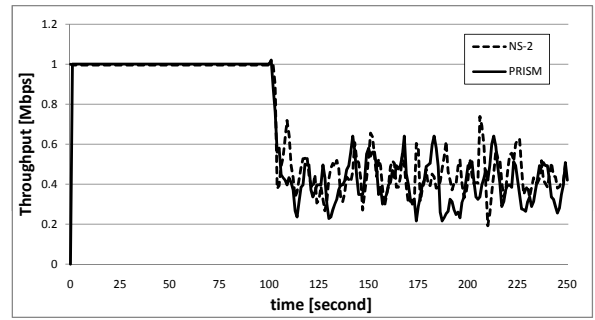
Figure 4: Comparison of the Throughput Obtained with NS-2 and PRISM
