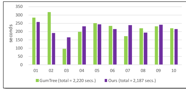
Fig. 10. Understanding time for the tasks
