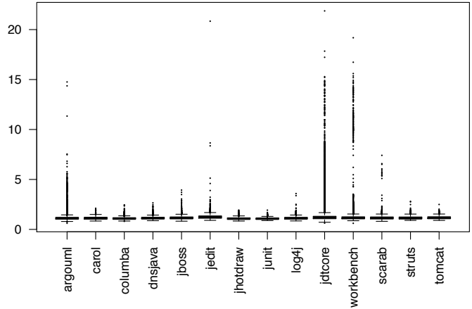
Fig. 9. Execution time ratio of our technique to GumTree
