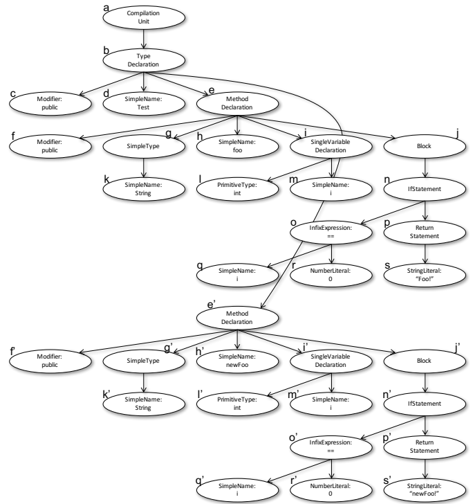
(b) Post-change AST
