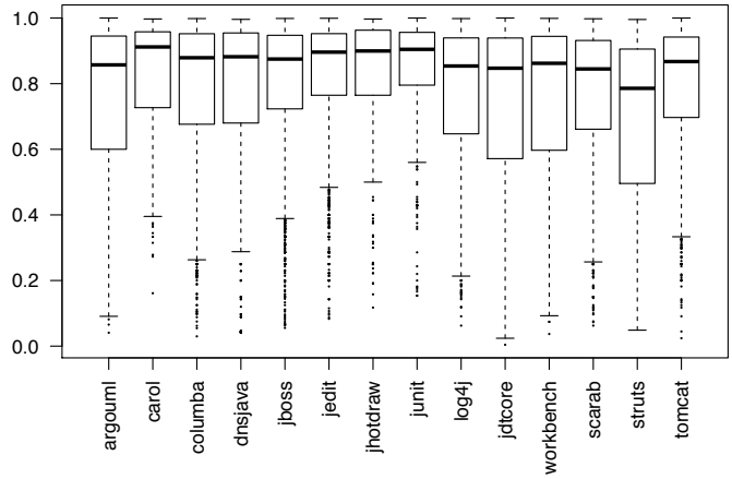
Fig. 8. Edit script length ratio of our technique to GumTree
